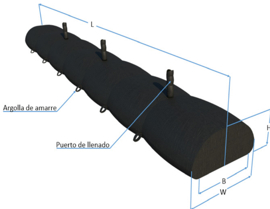
▲ Figura 17.3 | Geotextile Tube.
